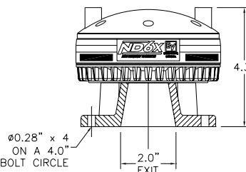
Side View (Shown with Optional ADH-6 Adapter)
